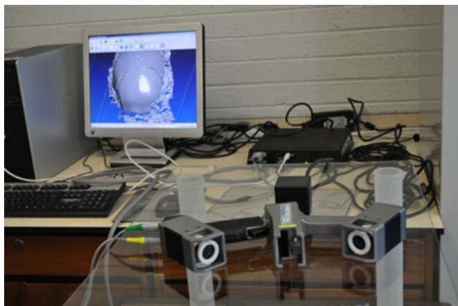
FIG. 1—The Polhemus FastSCAN Scorpion 3-D laser scanner. The double headed hand-held scanner is in the foreground, with the transmitter directly behind. The image on the screen is of a buried skull scanned in situ .
